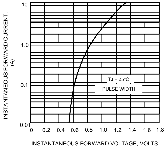
FIG.4-TYPICAL FORWARD CHARACTERISTICS
